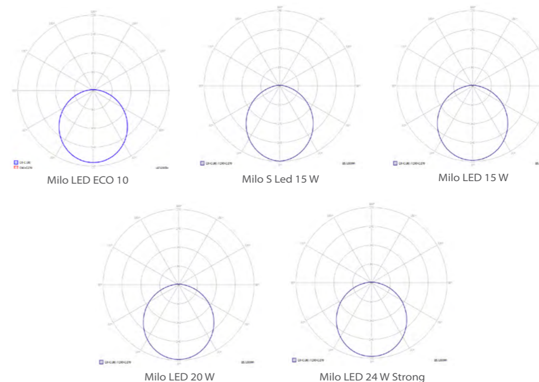
Milo LED
