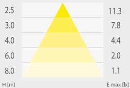
Suprema LED SCA 250
